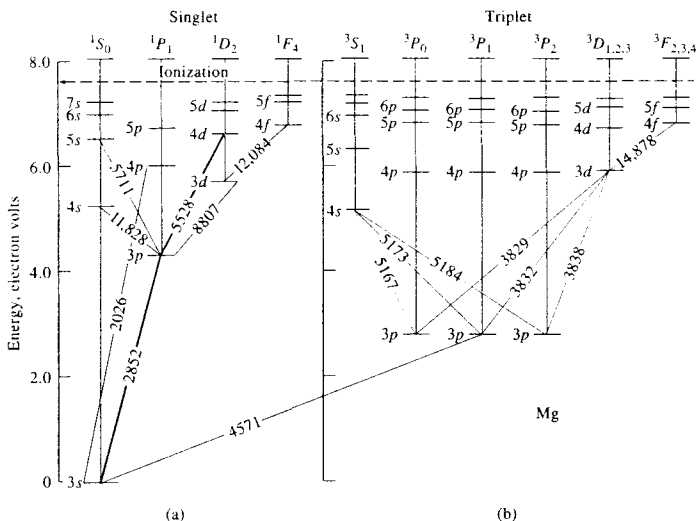
FIGURE 8-2 Energy diagram for atomic magnesium. The width of the lines between states indicates the relative line intensities. Note that a singlet-to-triplet transition is considerably less probable than a singlet-to-singlet transition. Wavelengths are presented in angstroms.
