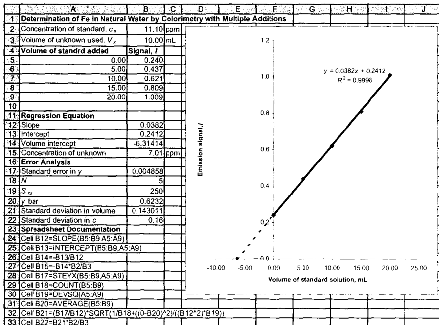
FIGURE 1-11 Spreadsheet for standard-addition Example 1-1.
