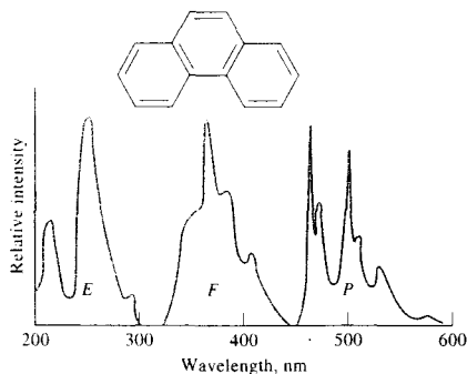
FIGURE 15-5 Spectra for phenanthrene: E , excitation; F , fluorescence; P , phosphorescence. (From W. R. Seitz, in Treatise on Analytical Chemistry , 2nd ed., P. J. Elving, E. J. Meehan, and I. M. Kolthoff, eds., Part I, Vol. 7, p. 169, New York: Wiley, 1981. Reprinted by permission of John Wiley & Sons, Inc.)
