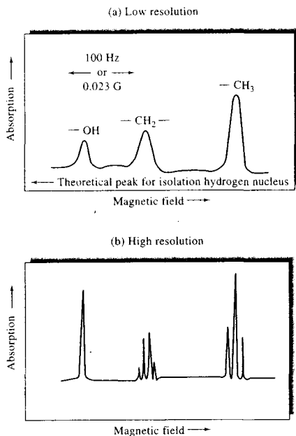
FIGURE 19-12 NMR spectra of ethanol at a frequency of 60 MHz. Resolution: (a) \sim 1/10^6 ; (b) \sim 1/10^7 .
