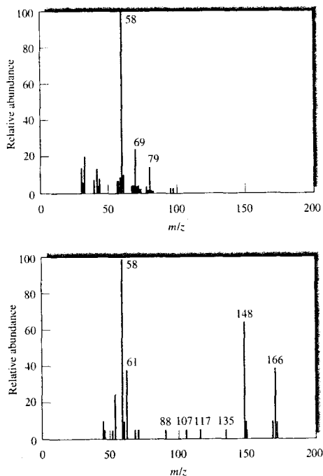
FIGURE 20-27 Electron-impact spectrum (a) and chemical ionization spectrum (b) of the same biologically important compound. (From H. M. Fales, H. A. Lloyd, and G. A. W. Milne, J. Amer. Chem. Soc. , 1970 , 92 , 1590–1597. American Chemical Society.)
