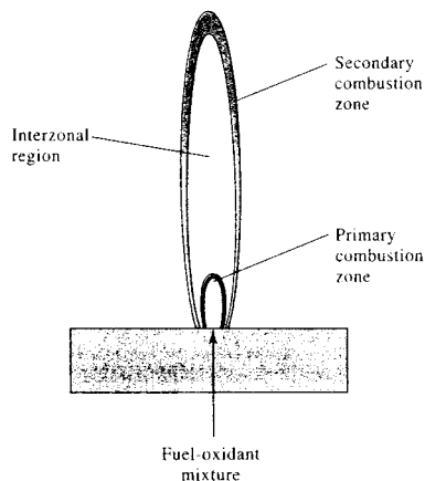
FIGURE 9-2 Regions in a flame.
