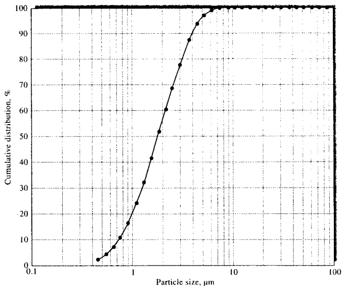
FIGURE 34-5 Cumulative undersize distribution.
