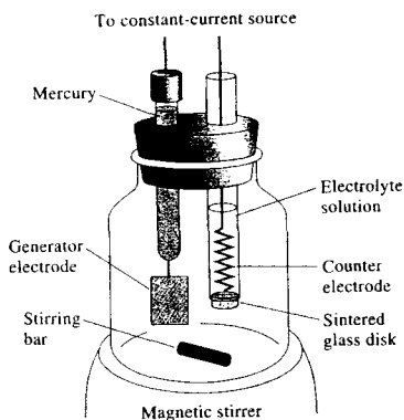
FIGURE 24-9 A typical coulometric titration cell.
