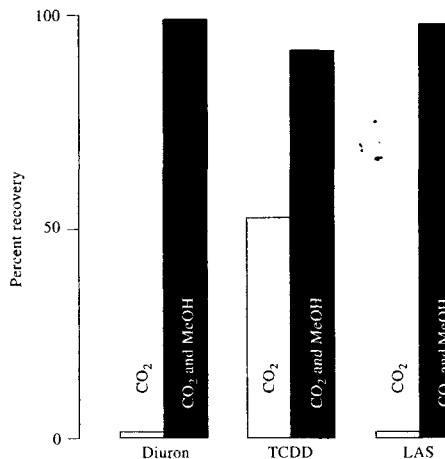
FIGURE 29-11 Comparison of extraction efficiencies obtained by using CO 2 and CO 2 modified with methanol. A soil sample was used. All extractions were for 30 min. Diuron is a common herbicide that is an aromatic substituted derivative of urea. TCDD is 2,3,7,8-tetrachlorodibenzo- p -dioxin. LAS is linear alkylbenzenesulfonate detergent.
