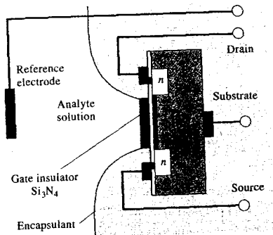
FIGURE 23-11 An ISFET for measuring pH.
