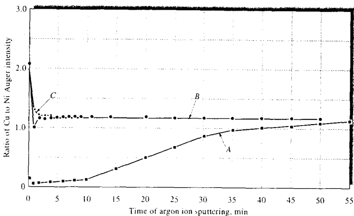
FIGURE 21-11 Auger sputtering profiles for the copper-nickel alloys shown in Figure 21-8: A , passivated sample; B , nonpassivated sample; C , chemically etched sample representing the bulk material. (Adapted from G. E. McGuire et al., J. Electrochem. Soc. , 1978 , 125, 1802. Reprinted by permission of the publisher, the Electrochemical Society, Inc.)
