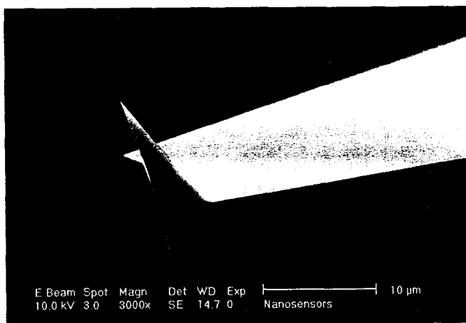
FIGURE 21-28 Micrograph of micromachined silicon cantilever and tip. (Courtesy of NanoWorld AG, Neuchatel, Switzerland.)
