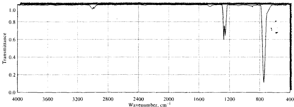
FIGURE 17-8 (a) Interferogram obtained from a typical FTIR spectrometer for methylene chloride. The plot shows detector signal output as a function of time or displacement of the moving mirror of the interferometer. (b) IR spectrum of methylene chloride produced by the Fourier transformation of the data in (a). Note that the Fourier transform takes signal intensity collected as a function of time and produces transmittance as a function of frequency after subtraction of a background interferogram and proper scaling.
