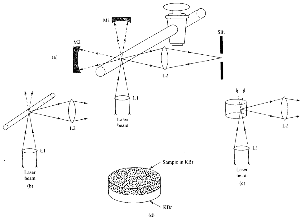
FIGURE 18-8 Sample illumination systems for Raman spectroscopy. In (a), a gas cell is shown with external mirrors for passing the laser beam through the sample multiple times. Liquid cells can be capillaries (b) or cylindrical cells (c). Solids can be determined as powders packed in capillaries or as KBr pellets (d).
