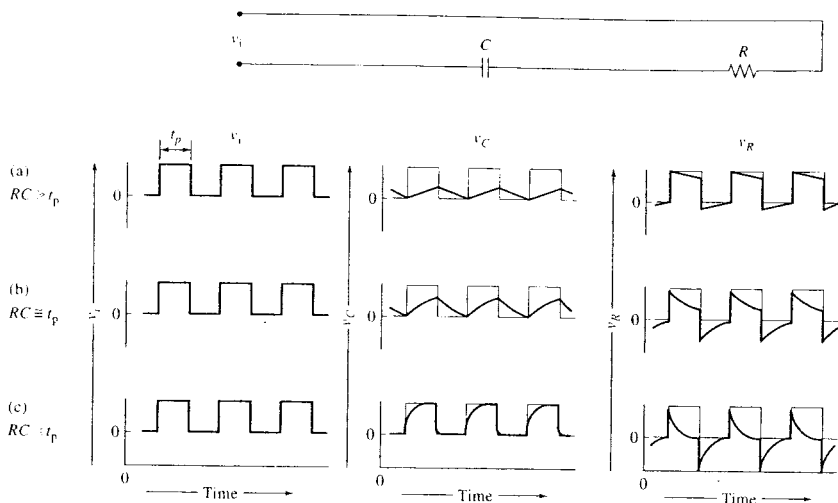
FIGURE 2-13 Output signals v_R and v_C for pulsed input signal v_i . (a) time constant \geq pulse width t_p ; (b) time constant = t_p ; (c) time constant \leq t_p .
