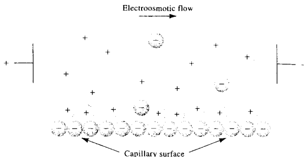
FIGURE 30-2 Charge distribution at a silica-capillary interface and resulting electroosmotic flow. (From A. G. Ewing, R. A. Wallingford, and T. M. Olefirowicz, Anal. Chem. , 1989 , 61 , 298A. Copyright 1989 American Chemical Society.)
