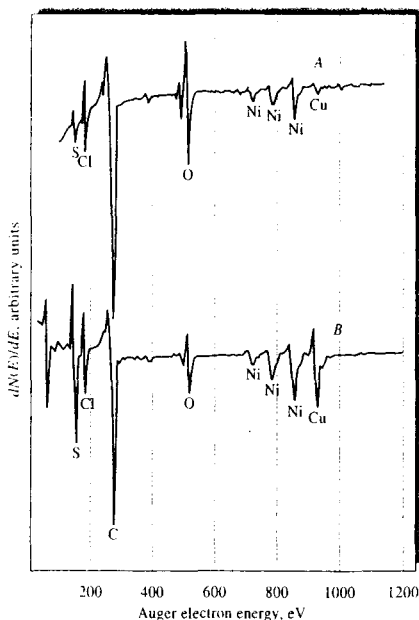
FIGURE 21-8 Auger electron spectra for a 70% Cu:30% Ni alloy. A , passivated by anodic oxidation; B , not passivated. (Adapted from G. E. McGuire et al., J. Electrochem. Soc. , 1978 , 125, 1802. Reprinted by permission of the publisher, the Electrochemical Society, Inc.)
