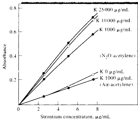
FIGURE 9-17 Effect of potassium concentration on the calibration curve for strontium. (Reprinted with permission from J. A. Bowman and J. B. Willis, Anal. Chem. , 1967 , 39 , 1220. Copyright 1967 American Chemical Society.)
