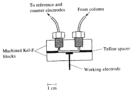
FIGURE 28-12 Amperometric thin-layer detector cell for HPLC.
