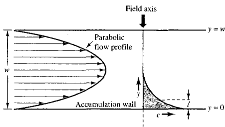
FIGURE 30-20 When the field is applied in FFF, components migrate to the accumulation wall where an exponential concentration profile exists as seen on the right. Components extend a distance y into the channel. The average thickness of the layer is l , which differs for each component. The main channel flow is then turned on and the parabolic flow profile of the eluting solvent is shown on the left.
