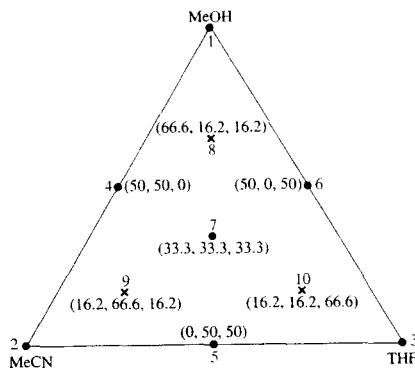
FIGURE 28-17 Solvent selectivity triangle for optimization of reversed-phase separations. Ten mixtures of the three organic solvents (methanol, acetonitrile, and tetrahydrofuran) are shown with the relative proportions indicated in parentheses (MeOH, MeCN, and THF). Water is used to maintain solvent strength and keep the k value within an appropriate range.
