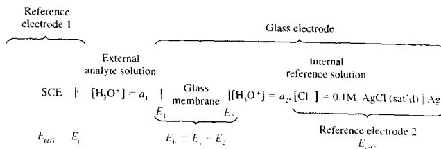
FIGURE 23-4 Diagram of glass-calomel cell for the measurement of pH. E_{\text{SCE}} is the potential of the reference electrode, E_1 is the junction potential, a_1 is the activity of hydronium ions in the analyte solution, E_1 and E_2 are the potentials on either side of the glass membrane, E_b is the boundary potential, and a_2 is the activity of hydronium ion in the internal reference solution.
