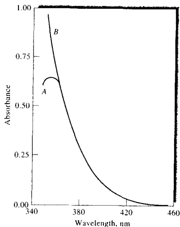
FIGURE 13-10 Spectrum of cerium(IV) obtained with a spectrophotometer having glass optics ( A ) and quartz optics ( B ). The false peak in A arises from transmission of stray radiation of longer wavelengths.
