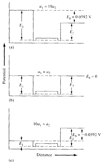
FIGURE 23-6 Potential profiles across a glass membrane from the analyte solution to the internal reference solution. The reference electrode potentials are not shown.
