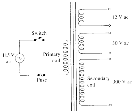
FIGURE 2-21 Schematic of a typical power transformer with multiple secondary windings.
