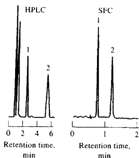
FIGURE 29-4 Comparison of chromatograms obtained by conventional partition chromatography (HPLC) and SFC. Column: 20 cm \times 4.6 mm with 10- \mu m reversed-phase bonded packing. Analytes: (1) biphenyl; (2) terphenyl. For HPLC: mobile phase, 65% CH 3 OH to 35% H 2 O; flow rate, 4 mL/min; linear velocity, 0.55 cm/s; sample size, 10 \mu L. For SFC: mobile phase, CO 2 ; flow rate, 5.4 mL/min; linear velocity, 0.76/s; sample size, 3 \mu L. (From D. R. Gere, T. J. Stark, and T. N. Tweeten, Application Note 800-4 , Hewlett-Packard Corp., Palo Alto, CA, 1983. With permission.)
