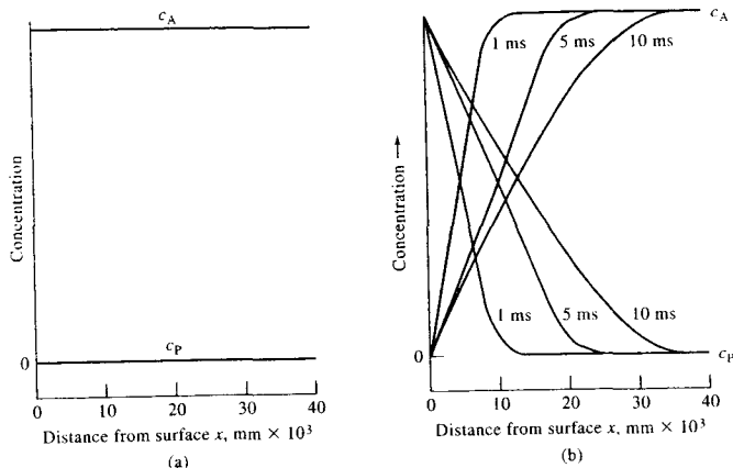
FIGURE 25-10 Concentration distance profiles during the diffusion-controlled reduction of A to give P at a planar electrode. (a) E_{\text{app}} = 0 V. (b) E_{\text{app}} = point Z in Figure 25-6; elapsed time: 1, 5, and 10 ms.
