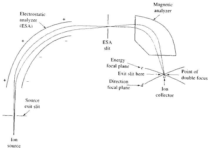
FIGURE 20-14 Nier-Johnson design of a double-focusing mass spectrometer.
