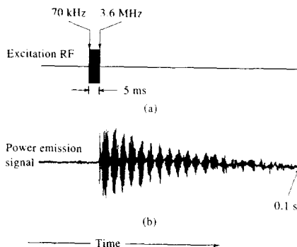
FIGURE 20-19 Schematic showing the timing of (a) the radio-frequency signal and (b) the transient image signal (lower). (Reprinted with permission from R. T. McIver Jr., Amer. Lab. , 1980, 12 (1), 26. Copyright 1980 by International Scientific Communications, Inc.)
