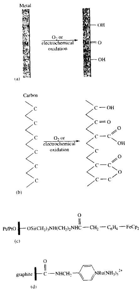
FIGURE 25-5 Functional groups formed on (a) a metal or (b) a carbon surface by oxidation. (With permission from A. J. Bard, Integrated Chemical Systems , New York: Wiley, 1994.) (c) A linking agent such as the organosilane shown is often bonded to the functionalized surface. Reactive components, such as ferrocenes, viologens, and metal bipyridine complexes, are then attached to form the modified surfaces. A Pt electrode is shown with a ferrocene attached. (With permission from J. R. Lenhard and R. W. Murray, J. Am. Chem. Soc. , 1978 , 100 , 7870.) In (d), a graphite electrode is shown with attached py-Ru(NH 3 ) 5 2+ . (With permission from C. A. Koval and F. C. Anson, Anal. Chem. , 1978 , 50 , 223.)
