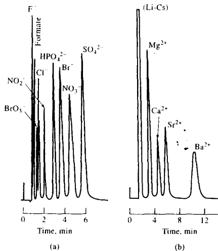
FIGURE 28-24 Typical applications of ion chromatography. (a) Separation of anions on an anion-exchange column. Eluent: 0.0028 M \text{NaHCO}_3 to 0.0023 M \text{Na}_2\text{CO}_3 . Sample size: 50 \mu\text{L} . (b) Separation of alkaline earth ions on a cation-exchange column. Eluent: 0.025 M phenylene diamine dihydrochloride to 0.0025 M HCl. Sample size: 100 \mu\text{L} . (Courtesy of Dionex Corp., Sunnyvale, CA.)
