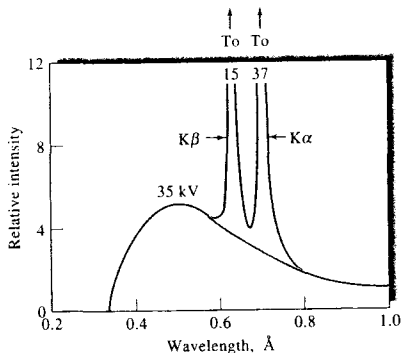
FIGURE 6-20 X-ray emission spectrum of molybdenum metal.
