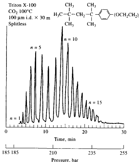
FIGURE 29-9 Chromatograms for the nonionic surfactant Triton X-100 with total current mass spectrometric detection. i.d. = inside diameter. (Reprinted with permission from R. D. Smith and H. R. Udseth, Anal. Chem. , 1987, 59, 17. Copyright 1981 American Chemical Society.)
