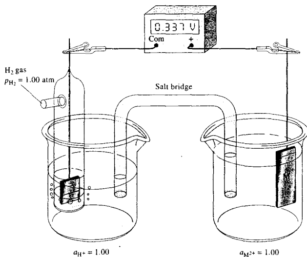
FIGURE 22-5 Measurement of the electrode potential for an M electrode. If the M^{2+} ion activity in the right-hand compartment is 1.00, the cell potential is the standard electrode potential of the half-reaction M^{2+}(aq) + 2e^- \rightleftharpoons M(s) .
