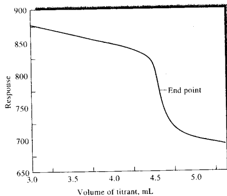
FIGURE 14-13 Photometric titration curves: (a) total hardness of water, (b) determination of sulfate. In (a), total water hardness is obtained by titration with 0.10 M EDTA at 610 nm for 100 mL of a solution that contained 2.82 mmol/L total hardness. Eriochrome Black T was the indicator. In (b), 10.0 mL of a solution containing sulfate was titrated with 0.050 M \text{BaCl}_2 using Thorin as an indicator and a wavelength of 523 nm. The response shown is proportional to transmittance. (From A. L. Underwood, Anal. Chem. , 1954, 26, 1322. Figure 1, p. 1323. Copyright 1954 American Chemical Society.)
