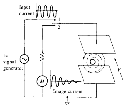
FIGURE 20-17 Path of an ion in a strong magnetic field. Inner solid line represents the original circular path of the ion. Dashed line shows spiral path when switch is moved briefly to position 1. Outer solid line is new circular path when switch is again opened.
