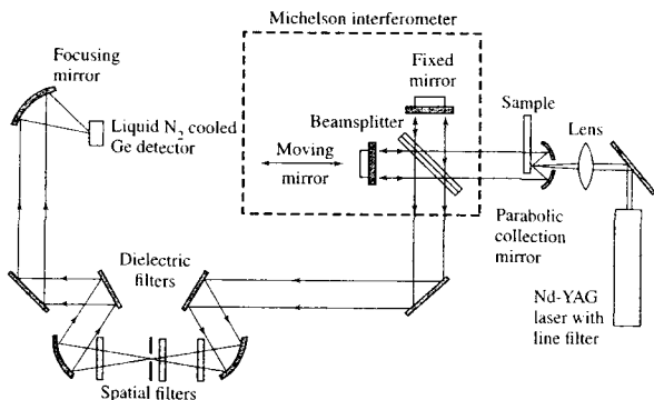
FIGURE 18-12 Optical diagram of an FT-Raman instrument. The laser radiation passes through the sample and then into the interferometer, consisting of the beam splitter and the fixed and movable mirrors. The output of the interferometer is then extensively filtered to remove stray laser radiation and Rayleigh scattering. After passing through the filters, the radiation is focused onto a cooled Ge detector.
