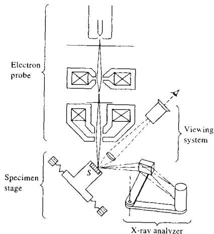
FIGURE 21-16 Schematic view of an electron microprobe. (From Wittr, Treatise on Analytical Chemistry , Kolthoff and Elving, Eds., Vol. 5, Part 1, p. 317B, New York: Interscience/Wiley, 1964.)
