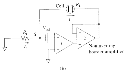
FIGURE 3-15 Constant-current sources.
