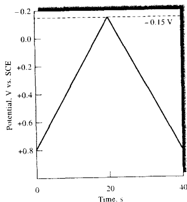
FIGURE 25-23 Cyclic voltammetric excitation signal.
