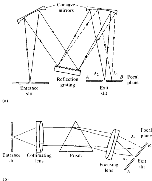
FIGURE 7-18 Two types of monochromators: (a) Czerny-Turner grating monochromator and (b) Bunsen prism monochromator. (In both instances, \lambda_1 > \lambda_2 .)
