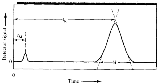
FIGURE 26-7 Determination of the number of plates
