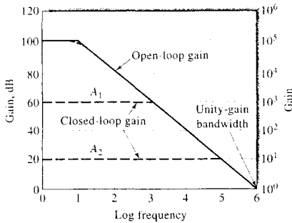
FIGURE 3-8 A Bode diagram showing the frequency response of a typical operational amplifier. Solid line: operational amplifier open-loop gain without negative feedback; dashed line: inverting amplifier configuration as in Figure 3-7 with A_1 = R_f/R_i = 1000 and A_2 = R_f/R_i = 10 .
