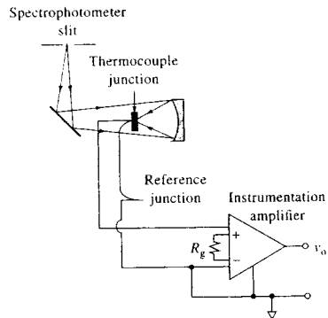
FIGURE 7-38 Thermocouple and instrumentation amplifier. The output voltage v_o is proportional to the thermocouple voltage. The magnitude of v_o is determined by the gain resistor R_g , which performs the same function as R_1/\mu in Figure 5-4.
