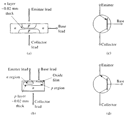
FIGURE 2-17 Two types of BJTs. Construction details are shown in (a) for a pnp alloy BJT and in (b) for an nnp planar transistor. Symbols for a pnp and nnp BJT are shown in (c) and (d), respectively. (Note that alloy junction transistors may also be fabricated as nnp types and planar transistors as pnp .)
