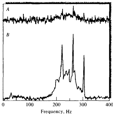
FIGURE 5-2 Effect of signal-to-noise ratio on the NMR spectrum of progesterone: A, S/N = 4.3 ; B, S/N = 43 . (Adapted from R. R. Ernst and W. A. Anderson, Rev. Sci. Inst. , 1966, 37, 101. With permission.)
