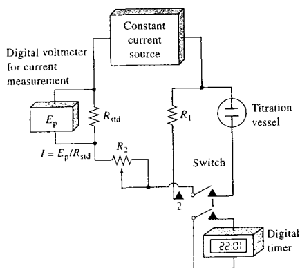
FIGURE 24-7 Schematic of a manual coulometric titration apparatus. Commercial coulometric titrators are totally electronic and usually computer controlled.
