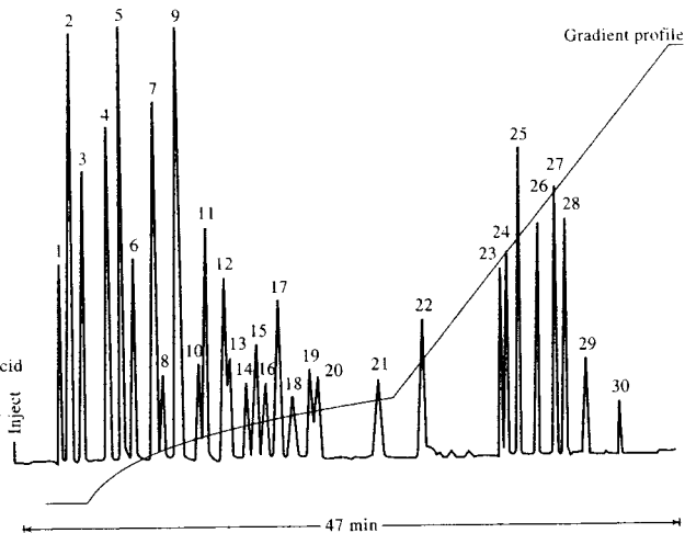
FIGURE 28-19 Chromatogram of orthophthalaldehyde derivatives of 30 amino acids of physiological importance. Column: 5\ \mu\text{m}\ \text{C}_{18} , reversed-phase. Solvent A: 0.05\ \text{M}\ \text{Na}_2\text{HPO}_4 , pH 7.4, 96:2:2\ \text{CH}_3\text{OH} , THF, \text{H}_2\text{O} . Fluorescence detector: excitation 334 nm; emission 425 nm. (Reprinted with permission from R. Pfeifer et al., Amer. Lab. , 1983 , 15 (3), 86. Copyright 1983 by International Scientific Communications, Inc.)
