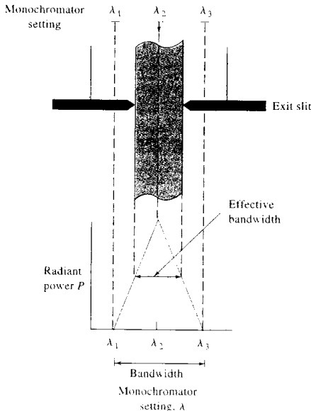
FIGURE 7-24 Illumination of an exit slit by monochromatic radiation \lambda_2 at various monochromator settings. Exit and entrance slits are identical.
