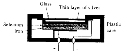
FIGURE 7-28 Schematic of a typical barrier-layer cell.
