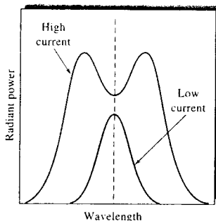
FIGURE 9-16 Emission line profiles for a hollow-cathode lamp operated at high and low currents.
