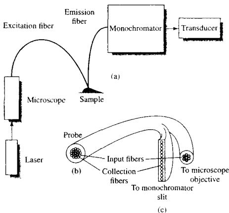
FIGURE 18-9 Raman spectrometer with fiber-optic probe. In (a) a microscope objective focuses the laser radiation onto excitation fibers that transport the beam to the sample. The Raman scattering is collected by emission fibers and carried to the entrance slit of a monochromator or to the entrance of an interferometer. A radiation transducer, such as a photomultiplier tube, converts the scattered light intensity to a proportional current or pulse rate; (b) end view of the probe; (c) end view of collection fibers at entrance slit of monochromator. The colored circles represent the input fiber and the uncolored circles the collection fibers. (Adapted from R. L. McCreery, M. Fleischmann, and P. Hendra, Anal. Chem. , 1983 , 55 , 146. Figure 1, p. 147. Copyright 1983 American Chemical Society.)
