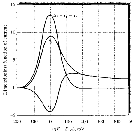
FIGURE 25-32 Current response for a reversible reaction to excitation signal in Figure 25-31c. This theoretical response plots a dimensionless function of current versus a function of potential, n(E - E_{1/2}) in millivolts. Here, i_1 = forward current; i_2 = reverse current; i_1 - i_2 = current difference. (From J. J. O'Dea, J. Osteryoung, and R. A. Osteryoung, Anal. Chem. , 1981 , 53 , 695. With permission Copyright 1981 American Chemical Society.)
