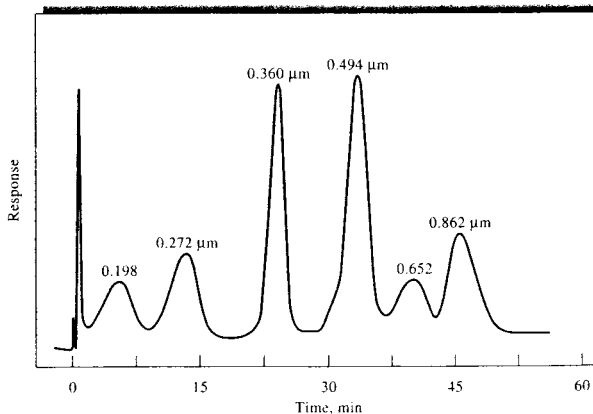
FIGURE 30-23 Fractogram illustrating separation of polystyrene beads of various diameters by sedimentation FFF. The channel flow rate was 2 mL/min. (Courtesy of FFFractionation, LLC, Salt Lake City, UT.)
