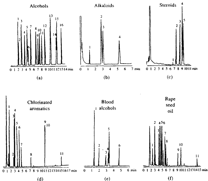
FIGURE 27-17 Typical chromatograms from open tubular columns coated with (a) polydimethyl siloxane; (b) 5% (phenyl methyl)dimethyl siloxane; (c) 50% (phenyl methyl)dimethyl siloxane; (d) 50% poly(trifluoropropyl-dimethyl) siloxane; (e) polyethylene glycol; (f) 50% poly(cyanopropyl-dimethyl) siloxane. (Courtesy of J&W Scientific.)
