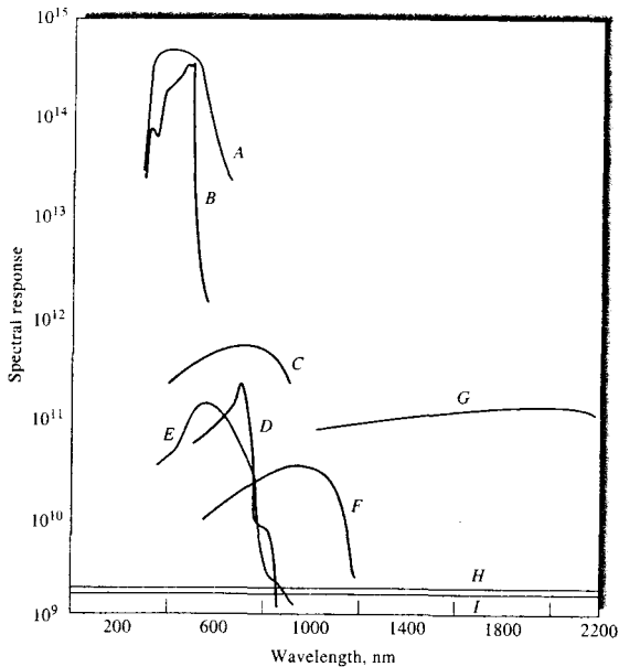
FIGURE 7-27 Relative response of various types of photoelectric transducers (A–G) and heat transducers (H, I): A, photomultiplier tube; B, CdS photoconductivity; C, GaAs photovoltaic cell; D, CdSe photoconductivity cell; E, Se/SeO photovoltaic cell; F, silicon photodiode; G, PbS photoconductivity; H, thermocouple; I, Golay cell. (Adapted from P. W. Druse, L. N. McGlauchlin, and R. B. Quistan, Elements of Infrared Technology , pp. 424–25, New York: Wiley, 1962. Reprinted by permission of John Wiley & Sons Inc.)
