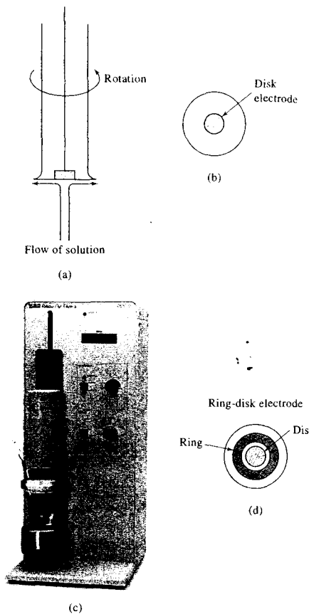
FIGURE 25-21 (a) Side view of an RDE showing solution flow pattern. (b) Bottom view of a disk electrode. (c) Photograph of a commercial RDE. (Courtesy of Bioanalytical Systems, Inc., West Lafayette, IN.) (d) Bottom view of a ring-disk electrode.
