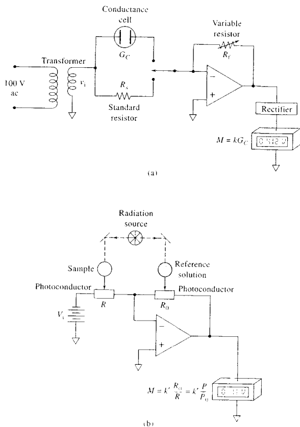
FIGURE 3-12 Two circuits for transducers whose conductance or resistance is the quantity of interest. (a) The output of the cell is a current proportional to the conductance of the electrolyte. (b) The ratio of the resistances of the photoconductive cells is proportional to the meter reading.
