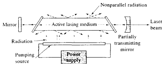
FIGURE 7-4 Schematic representation of a typical laser source.
