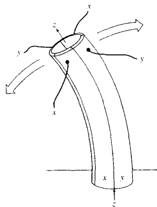
FIGURE 21-25 Piezoelectric scanner of the segmented tube design.
