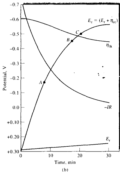
FIGURE 24-1 Changes in (a) current and (b) potentials during the electrolytic deposition of \text{Cu}^{2+} . Points A and B on the cathode potential curve are potentials at which Pb and Cd would begin to codeposit if present. Point C is the potential at which \text{H}_2 might begin to form at the cathode. Any of these processes would distort curve ABC.
