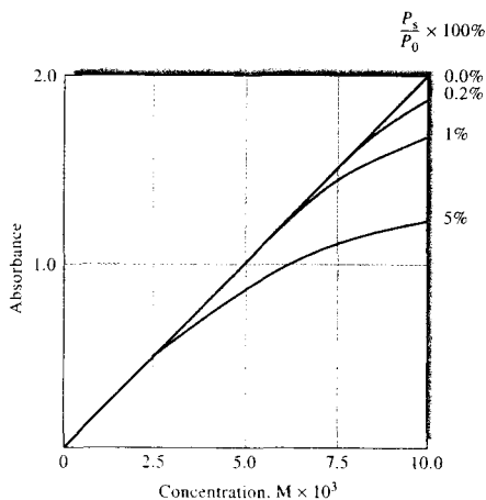
FIGURE 13-6 Apparent deviation from Beer's law brought about by various amounts of stray radiation. Note that the absorbance begins to level off with concentration at high stray-light levels. Stray light always limits the maximum absorbance that can be obtained because when the absorbance is high, the radiant power transmitted through the sample can become comparable to or lower than the stray-light level.
