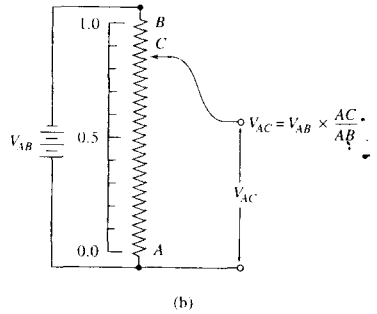
FIGURE 2-2 Voltage dividers: (a) fixed attenuator type and (b) continuously variable type (potentiometer).
