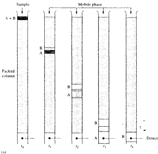
FIGURE 26-1 (a) Diagram showing the separation of a mixture of components A and B by column elution chromatography. (b) The output of the signal detector at the various stages of elution shown in (a).
