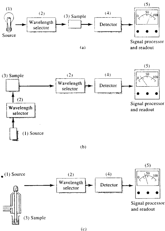
FIGURE 7-1 Components of various types of instruments for optical spectroscopy. In (a), the arrangement for absorption measurements is shown. Note that source radiation of the selected wavelength is sent through the sample, and the transmitted radiation is measured by the detector–signal processing–readout unit. With some instruments, the position of the sample and wavelength selector is reversed. In (b), the configuration for fluorescence measurements is shown. Here, two wavelength selectors are needed to select the excitation and emission wavelengths. The selected source radiation is incident on the sample and the radiation emitted is measured, usually at right angles to avoid scattering. In (c), the configuration for emission spectroscopy is shown. Here, a source of thermal energy, such as a flame or plasma, produces an analyte vapor that emits radiation isolated by the wavelength selector and converted to an electrical signal by the detector.
