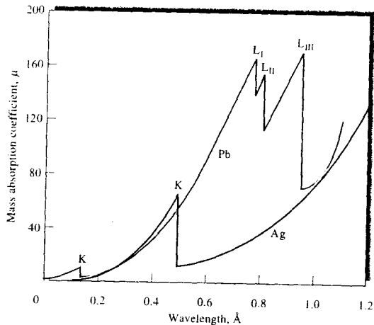
FIGURE 12-5 X-ray absorption spectra for lead and silver.
