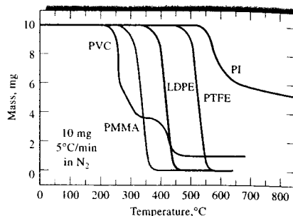
FIGURE 31-3 Thermograms for some common polymer materials. PVC = polyvinyl chloride; PMMA = polymethyl methacrylate; LDPE = low-density polyethylene; PTFE = polytetrafluoroethylene; PI = aromatic polypyromellitimide. (From J. Chiu, in Thermoanalysis of Fiber-Forming Polymers , R. F. Schwenker, ed., New York: Wiley, 1966.)
