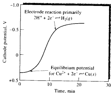
FIGURE 24-2 Changes in cathode potential during the deposition of copper with a constant current of 1.5 A. The cathode potential is equal to E_r + \eta_{tc} .
