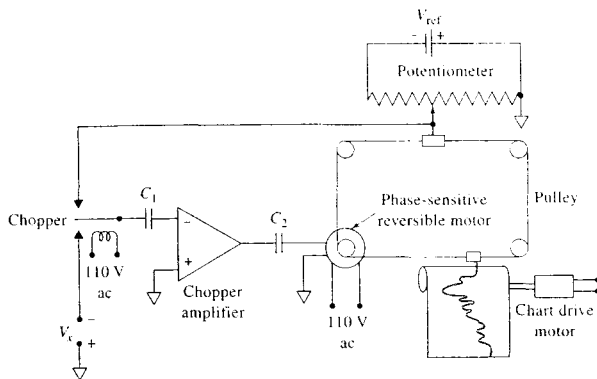
FIGURE 2-27 Schematic of self-balancing recording potentiometer.
