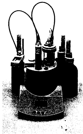
FIGURE 24-8 An automated coulometric titrator. All instrument functions are under control of an internal computer, and results of determinations appear on the LCD display. (Courtesy of Mettler-Toledo, Inc., Columbus, OH.)
