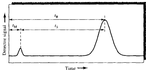
FIGURE 26-4 A typical chromatogram for a two-component mixture. The small peak on the left represents a solute that is not retained on the column and so reaches the detector almost immediately after elution is begun. Thus, its retention time t_M is approximately equal to the time required for a molecule of the mobile phase to pass through the column.
