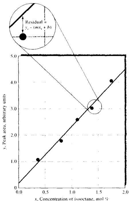
FIGURE 1-8 Calibration curve for the determination of isoctane in a hydrocarbon mixture. The residual is the difference between an experimental data point y , and that calculated from the regression model, mx_i + b , as shown in the insert.
