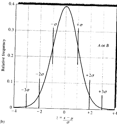
FIGURE a1-3 Normal error curves. The standard deviation of B is twice that of A ; that is, \sigma_B = 2\sigma_A . (a) The abscissa is the deviation from the mean in the units of the measurement. (b) The abscissa is the deviation from the mean relative to \sigma . Thus, A and B produce identical curves when the abscissa is z = (x - \mu) / \sigma .
