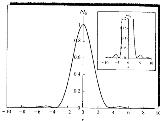
FIGURE 34-3 The Airy function showing a plot of intensity I relative to the central intensity I_0 as a function of the variable x (see text). The inset shows an expansion of the y -axis to show the maxima and minima more clearly.
