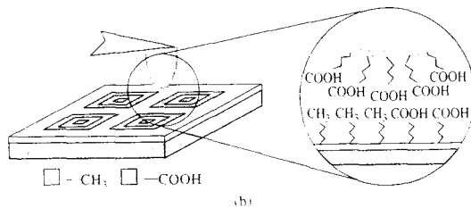
FIGURE 21-31 Detection of a functional group by atomic force microscopy. (a) Carboxylic acid groups are chemically attached to a gold-coated AFM tip. (b) Schematic views of the experiment. (Inset) Interaction between the gold tip coated with -\text{COOH} groups and the sample coated with both -\text{CH}_3 and -\text{COOH} groups. (Adapted from C. D. Frisbie, L. F. Rozsnyai, A. Noy, M. S. Wrighton, and C. M. Lieber, Science , 1994 , 265, 2072. With permission.)
