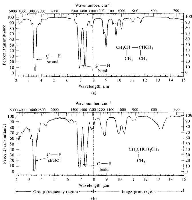
FIGURE 17-5 The group frequency region of the mid-IR ( \sim 3600 – 1250\text{ cm}^{-1} ) is used to identify common functional groups. The fingerprint region ( \sim 1200 – 600\text{ cm}^{-1} ) is used to identify compounds. (From R. M. Roberts, J. C. Gilbert, L. B. Rodewald, and A. S. Wingrove, Modern Experimental Organic Chemistry , 4th ed., Philadelphia: Saunders, 1985. With permission.)
