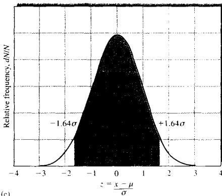
FIGURE a1-5 Areas under a Gaussian curve for various values of \pm z . (a) z = \pm 0.67 ; (b) z = \pm 1.29 ; (c) z = \pm 1.64 ; (d) z = \pm 1.96 ; (e) z = \pm 2.58 .
