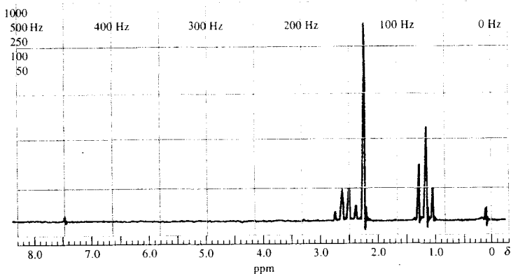
FIGURE 19-41 Proton NMR spectrum. (Courtesy of Varian, Inc., Palo Alto, CA.)
