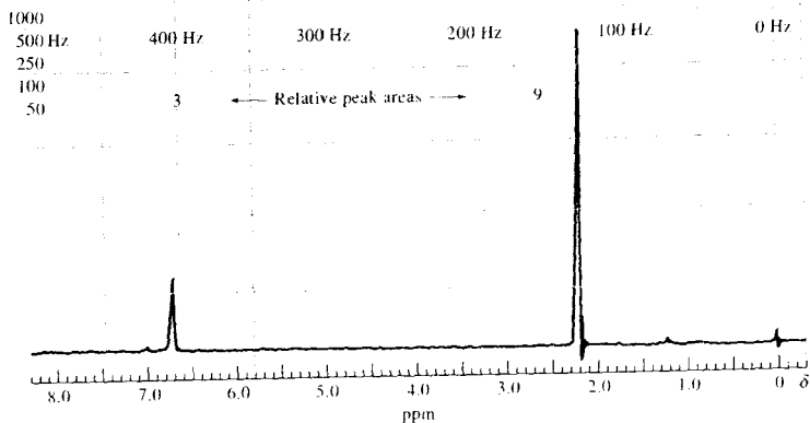
FIGURE 19-25 NMR spectra for two organic isomers in CDCl_3 . (Courtesy of Varian Inc., Palo Alto, CA.)
