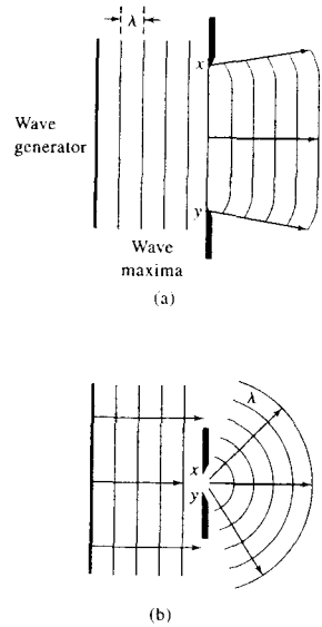
FIGURE 6-7 Propagation of waves through a slit: (a) xy \gg \lambda ; (b) xy = \lambda .
