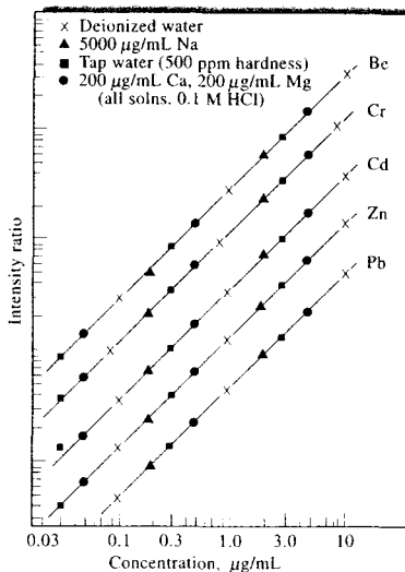
FIGURE 10-16 Internal standard calibration curves with an ICP source. Here, a yttrium line at 242.2 nm served as an internal standard. Notice the lack of interelement interference. (From V. A. Fassel, Science , 1978 , 202 , 187. With permission. Copyright 1978 by the American Association for the Advancement of Science.)
