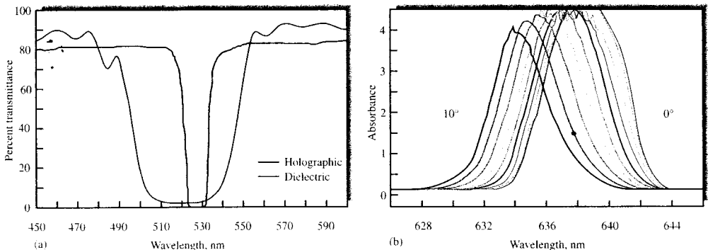
FIGURE 7-15 (a) Comparison of the bandwidths of a typical holographic notch filter and an interference filter. (b) Tilt-tuning of a holographic notch filter by 1^\circ increments from perpendicular to the incident laser beam. The rejection band can be finely adjusted by altering the angle of the notch filter relative to the laser. (Courtesy of Kaiser Optical Systems, Inc., Ann Arbor, MI, with permission.)
