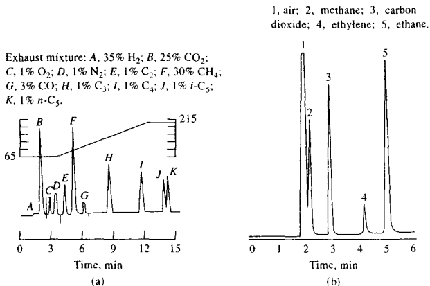
FIGURE 27-21 Typical gas-solid chromatographic separations: (a) a 5 ft. \times 1/8 in. molecular sieve column; (b) a 30 m \times 0.53 mm PLOT column. C_n = hydrocarbon with n carbons.
