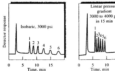
FIGURE 29-2 Effect of pressure programming in SFC. Note the shorter time for the pressure-gradient chromatogram on the right compared with the constant pressure (isobaric) chromatogram on the left. (Courtesy of Brownlee Labs, Santa Clara, CA.)
