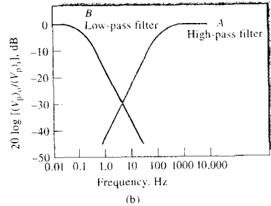
FIGURE 2-12 (a) Frequency response of high-pass and low-pass filters. (b) Bode diagram for high-pass and low-pass filters. For the high-pass filter, R = 10 \text{ k}\Omega and C = 0.1 \text{ }\mu\text{F} . For the low-pass filter, R = 1 \text{ M}\Omega and C = 1 \text{ }\mu\text{F} .
