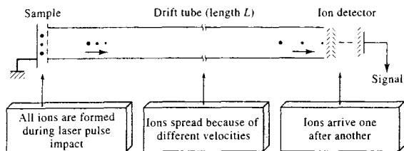
FIGURE 11-10 Principle of a TOF mass spectrometer. A spatially tightly bunched group of ions produced by a laser probe is accelerated into the drift tube where separation occurs. (From A. H. Verbeuken, F. J. Bruynseels, R. Van Grieken, and F. Adams, in Inorganic Mass Spectrometry , p. 186, F. Adams, R. Gijbels, and R. Van Grieken, eds., New York: Wiley, 1988. With permission.)
