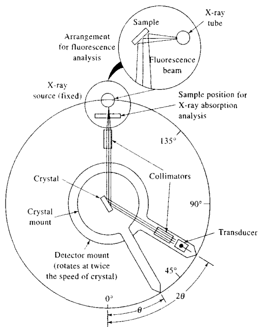
FIGURE 12-9 An X-ray monochromator and detector. Note that the angle of the detector with respect to the beam ( 2\theta ) is twice that of the crystal face. For absorption analysis, the source is an X-ray tube and the sample is located in the beam as shown. For emission measurements, the sample becomes a source of X-ray fluorescence as shown in the insert.
