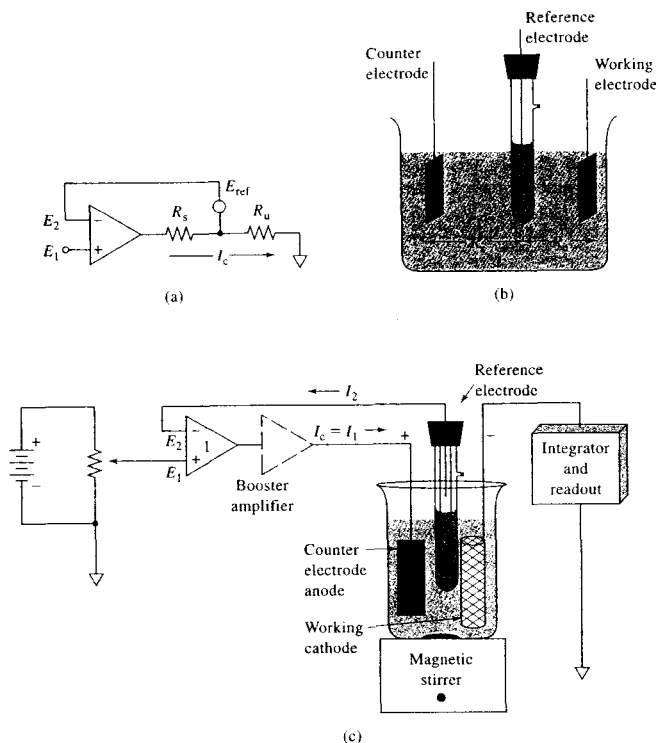
FIGURE 24-6 Schematic of a system for controlled-potential coulometry. (a) Equivalent circuit. (b) Resistances within the cell. (c) Practical circuit. The cell current I_c passes to the integrator-readout module, which provides a number proportional to the total quantity of charge that passes through the cell.
