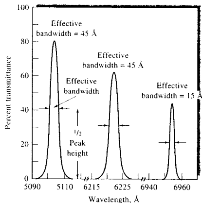
FIGURE 7-13 Transmission characteristics of typical interference filters.
