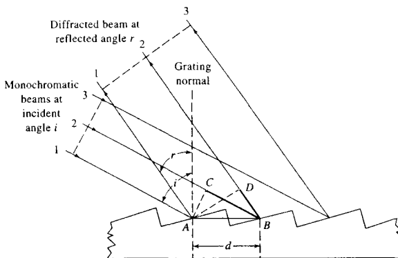
FIGURE 7-21 Mechanisms of diffraction from an echellette-type grating.
