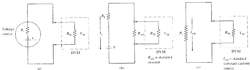
FIGURE 2-4 Uses of a DVM. (a) Measurement of the output V_s of a voltage source. (b) Measurement of current I_s through a load resistor R_L . (c) Measurement of resistance R_x of a resistive circuit element.
