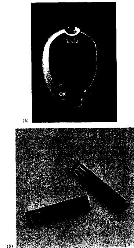
FIGURE 33-19 Photograph of a blood glucose monitor for in-home use. The meter (a) contains the electronics and display. A droplet of blood is placed on a test strip (b), which is placed at the top of the meter. The test strip contains immobilized glucose oxidase and electrodes for the amperometric detection system. (Courtesy of Life-Scan, Inc., Milpitas, CA.)
