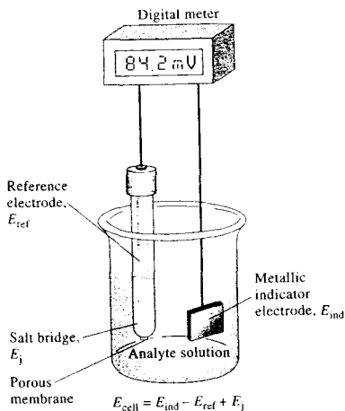
FIGURE 23-1 A cell for potentiometric determinations.
