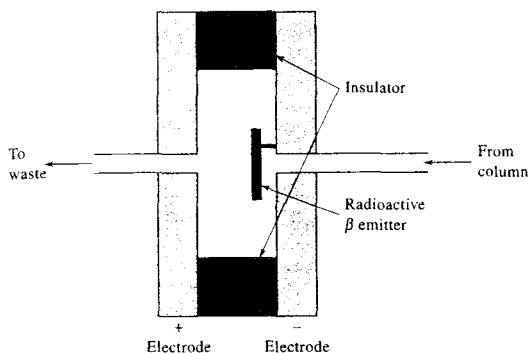
FIGURE 27-10 Schematic diagram of an ECD.
