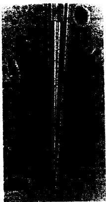
FIGURE 23-10 Photograph of a potassium liquid-ion exchanger (valinomycin) microelectrode with 125 nm of ion exchanger inside the tip. The magnification of the original photo was 400 \times . (From J. L. Walker, Anal. Chem. , 1971 , 43 [3], 91A. Reproduced by permission of the American Chemical Society.)
