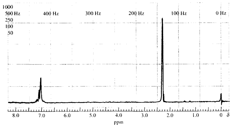
FIGURE 19-43 Proton NMR spectra. (Courtesy of Varian, Inc., Palo Alto, CA.)
