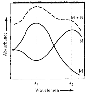
FIGURE 14-9 Absorbance spectrum of a two-component mixture (M + N) with spectra of the individual components. Vertical dashed lines indicate optimal wavelengths for determination of the two components.
