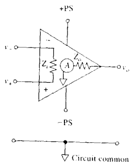
FIGURE 3-1 Equivalent circuit representation of an operational amplifier.
