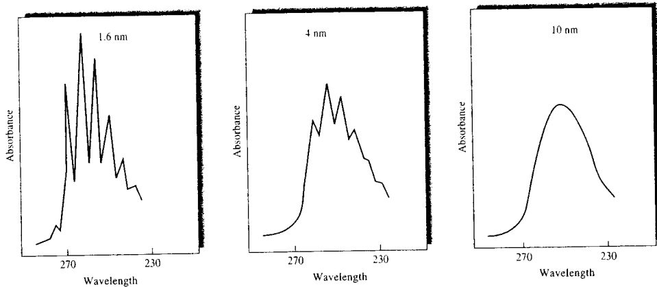
FIGURE 13-8 Effect of bandwidth on spectral detail for a sample of benzene vapor. Note that as the spectral bandwidth increases, the fine structure in the spectrum is lost. At a bandwidth of 10 nm, only a broad absorption band is observed.
