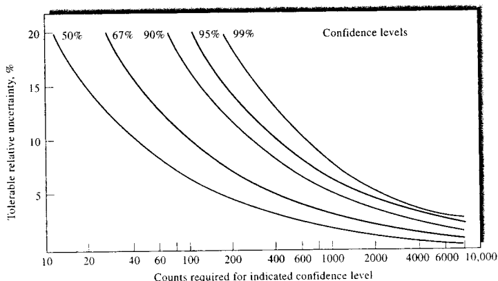
FIGURE 32-2 Relative uncertainty in counting.
