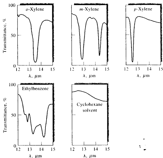
FIGURE 17-10 Spectra of C_8H_{10} isomers in cyclohexane.
