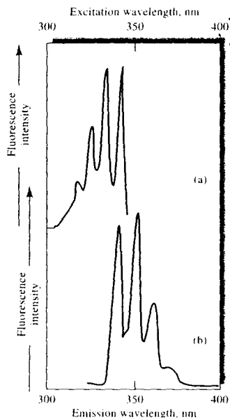
FIGURE 15-9 Fluorescence spectra for 1 ppm anthracene in alcohol: (a) excitation spectrum; (b) emission spectrum.
