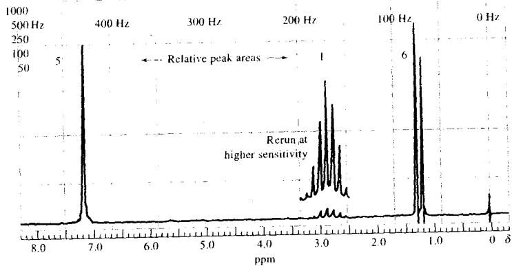
FIGURE 19-24 NMR spectrum and peak integral curve for the organic compound C_9H_{10}O_2 in CCl_4 . (From R. M. Silverstein, G. C. Bassler, and T. C. Morrill, Spectrometric Identification of Organic Compounds , 3rd ed., p. 296, New York: Wiley, 1974. With permission.)
