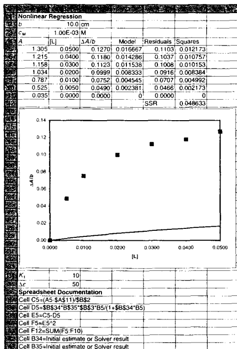
FIGURE 14-21 Spreadsheets to calculate formation constants using nonlinear regression. (a) The results from the model (Equation 14-10) are calculated in column D using the initial estimates of K_f = 10 and \Delta\epsilon = 50 . The plot shows the model values (solid line) and the data values (points). The difference between the data values (column C) and the model values (column D) are the residuals shown in column E. The squares of these are calculated in column F and summed in cell F12 (SSR). In (b), Excel's Solver has minimized the value in cell F12 to obtain the best-fit values shown in cells B34 and B35. The model values are again shown as the solid line in the plot.
