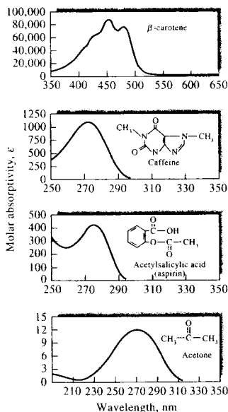
FIGURE 14-2 Absorption spectra for typical organic compounds.
