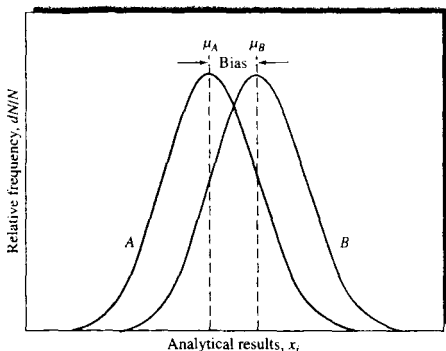
FIGURE a1-2 Illustration of systematic error in analytical results. Curve A is the frequency distribution for the accepted value by Method A , which has no bias. Curve B illustrates the distribution of results by Method B , which has a significant bias = \mu_B - \mu_A .
