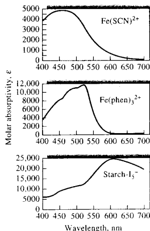
FIGURE 14-5 Absorption spectra of aqueous charge-transfer complexes.
