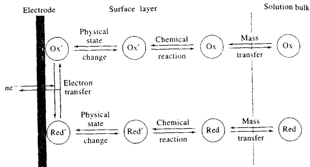
FIGURE 22-8 Steps in the reaction \text{Ox} + ne^- \rightleftharpoons \text{Red} at an electrode. Note that the surface layer is only a few molecules thick. (Adapted from A. J. Bard and L. R. Faulkner, Electrochemical Methods , 2nd ed., p. 23, New York: Wiley, 2001. Reprinted by permission of John Wiley & Sons, Inc.)
