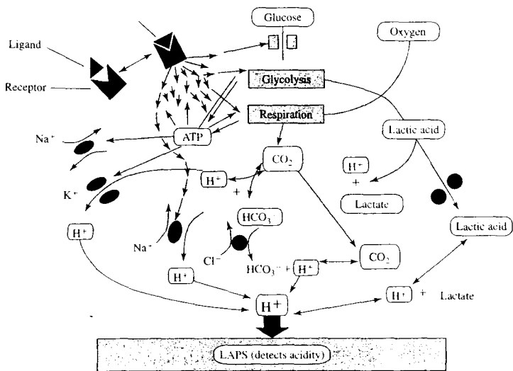
FIGURE IA4-1 The cell biology of extracellular acidification. When a receptor is stimulated, signal transduction pathways are induced. Adenosine triphosphate (ATP) consumption is then compensated by the increased uptake and metabolism of glucose, which results in an increase in the excretion of acid waste products. The extracellular acidification is measured by the LAPS. (From F. Hafner, Biosens. Bioelectron. , 2000, 15, 149. With permission.)
