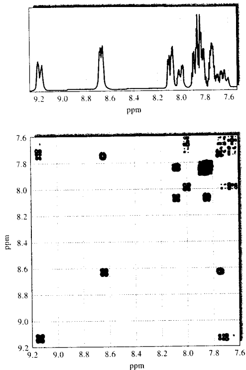
FIGURE 19-47 300-MHz COSY spectrum of phenanthro[3,4-b]thiophene. (From J. B. Lambert and E. P. Mazzola, Nuclear Magnetic Resonance Spectroscopy , Upper Saddle River, NJ: Pearson/Prentice-Hall, 2004. With permission.)
