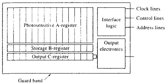
FIGURE 10-12 Schematic of an array segment showing phototransducers, storage and output registers, and readout circuitry. (From T. W. Barnard et al., Anal. Chem. , 1993 , 65 , 1231. Figure 3, p. 1232. Copyright 1993 American Chemical Society.)
