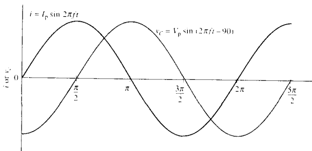
FIGURE 2-9 Sinusoidal current i and voltage v_C signals for a capacitor.
