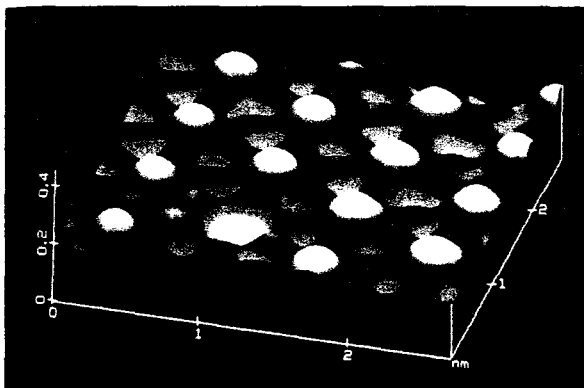
FIGURE 21-29 STM scan of iodine atoms in a 3\text{-nm} \times 3\text{-nm} array adsorbed on platinum. Note the missing iodine atom in the bottom center of the image. (Image provided by Veeco Instruments.)
