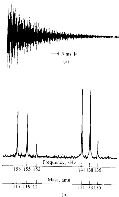
FIGURE 20-20 Time-domain (a) and (b) frequency- or mass-domain spectrum for 1,1,1,2-tetrachloroethane. (Reprinted with permission from E. B. Ledford Jr. et al., Anal. Chem. , 1980, 52, 463. Copyright 1980 American Chemical Society.)
