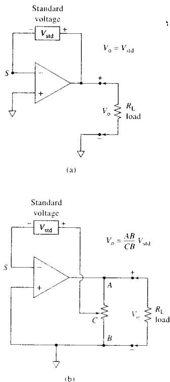
FIGURE 3-14 Constant-voltage sources.
