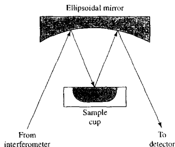
FIGURE 17-11 A diffuse-reflectance attachment for an FTIR spectrometer.
