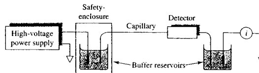
FIGURE 30-1 Schematic of a capillary electrophoresis system.
