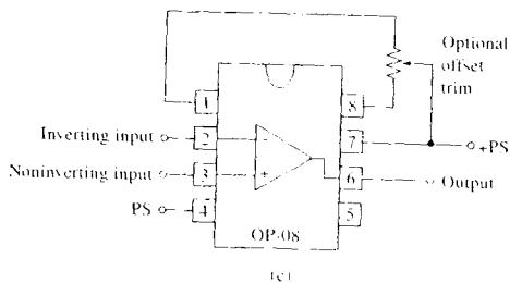
FIGURE 3-2 Symbols for operational amplifiers. More detail than usual is provided in (a). Note that the two input voltages v_i and v_n , as well as the output voltage v_o , are measured with respect to the circuit common, which is usually at or near earth ground potential. (b) The usual way of representing an operational amplifier in circuit diagrams. (c) Representation of typical commercial 8-pin operational amplifier.
