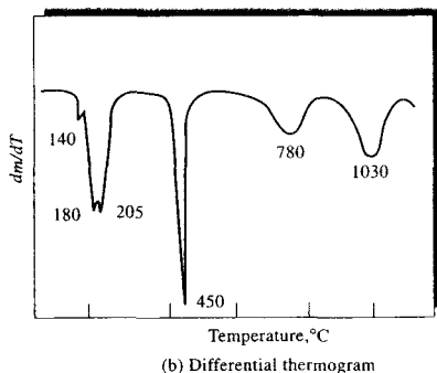
FIGURE 31-6 Decomposition of \text{CaC}_2\text{O}_4 \cdot \text{H}_2\text{O} , \text{SrC}_2\text{O}_4 \cdot \text{H}_2\text{O} , and \text{BaC}_2\text{O}_4 \cdot \text{H}_2\text{O} . From L. Erdey, G. Liptay, G. Svehla, and F. Paulike, Talanta , 1962 , 9 , 490. With permission.)
