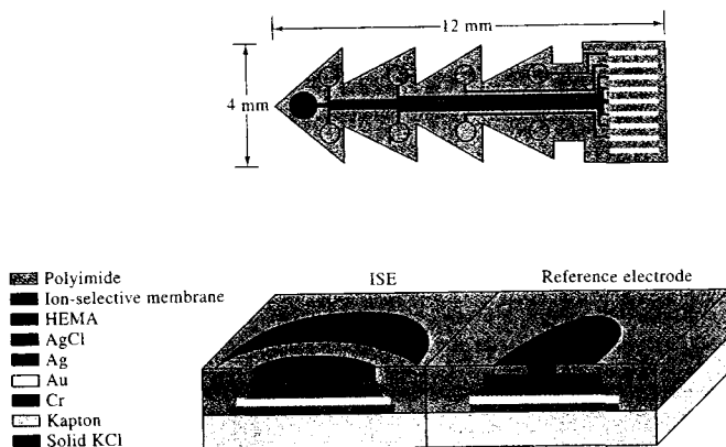
FIGURE 23-15 A microfabricated potentiometric sensor for in vivo determination of analytes. The sensor was fabricated on a flexible plastic substrate using thick-film techniques. There are nine ion-selective electrodes (ISEs) on one side of the film and corresponding reference electrodes on the opposite side. (From E. Lindner and R. P. Buck, Anal. Chem. , 2000 , 72 , 336A, with permission. Copyright 2000 American Chemical Society.)
