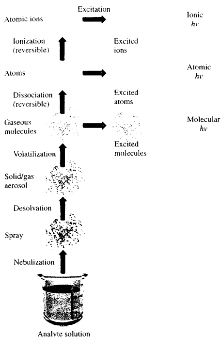
FIGURE 9-1 Processes occurring during atomization.
