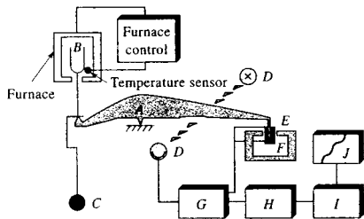
FIGURE 31-1 Thermobalance components. The balance beam is shown as A . The sample cup and holder are B ; C is a counterweight. D is a lamp and photodiodes, E is a magnetic coil, and F is a permanent magnet. The computer data-acquisition, data-processing, and control systems are components G , H , and I . Component J is the printer and display unit. (Courtesy of Mettler-Toledo.)
