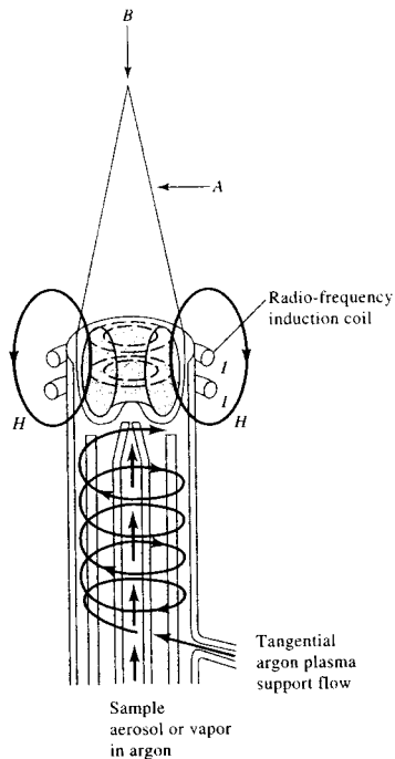
FIGURE 10-1 A typical ICP source. Position A shows radial viewing of the torch, and position B shows axial viewing. (From V. A. Fassel, Science , 1978 , 202 , 185. With permission. Copyright 1978 by the American Association for the Advancement of Science.)
