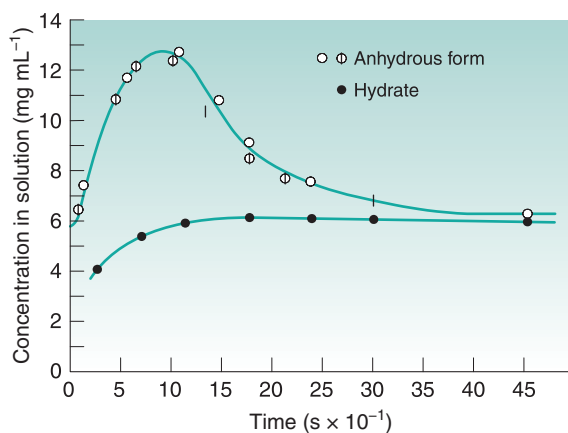
Figure 8.4 • The dissolution of theophylline monohydrate rising to an equilibrium solubility, compared with that for anhydrous theophylline, which forms a supersaturated solution with a peak more than twice that of the dissolving hydrate, before crystallizing to form the true equilibrium solubility. Adapted from Shefter & Higuchi, 1963, with permission.
