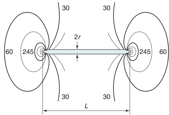
Fig. 10.1 • Stress concentrations at the edges of a disc-shaped crack; r is the radius of curvature of the crack tip and L is the crack length.
