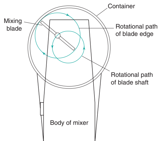
Fig.11.11 • Top view of a planetary mixer, showing the path of the paddle.
