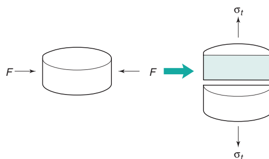
Fig. 30.22 • The tensile failure of a tablet during diametral compression.
