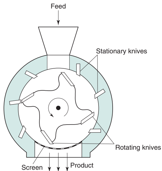
Fig. 10.6 • Cutter mill.
