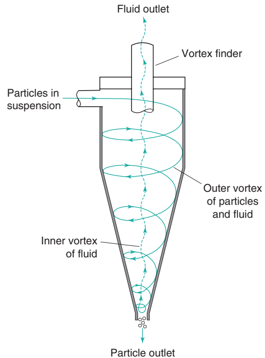
Fig. 10.23 • Reverse-flow cyclone separation.
