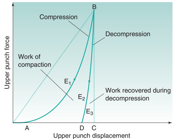
Fig. 30.26 • The relationship between upper punch force and upper punch displacement during compression and decompression of a powder. Adapted from Ragnarsson, 1996.
