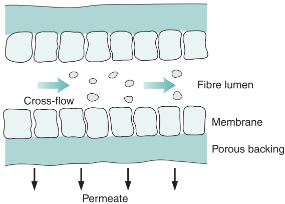
Fig. 25.6 • Cross-flow microfiltration through an individual fibre.
