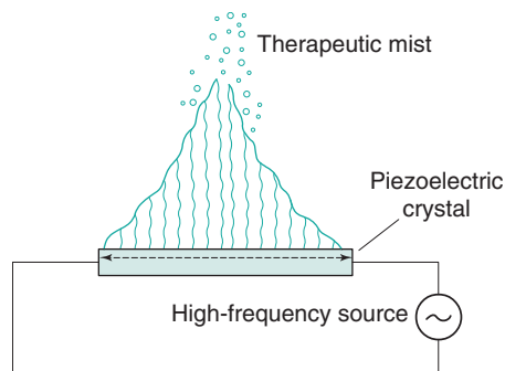
Fig. 37.9 • An ultrasonic nebulizer.
