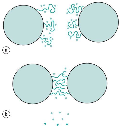
Fig. 5.8 • Enthalpic stabilization. (a) Particles with stabilizing polyoxyethylene chains and hydrogen-bonded water molecules. (b) Stabilizing chains overlap, water molecules released, resulting in positive \Delta H .
