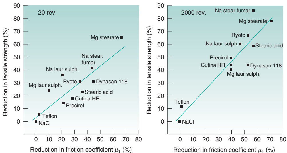
Fig. 30.9 • The reduction in tablet tensile strength as a function of the reduction in friction coefficient during tableting of a sodium chloride powder mixed with 0.1% by weight of a series of lubricants admixed at two different mixing intensities. Mg laur sulph. , magnesium lauryl sulfate; Mg stearate , magnesium stearate; Na laur sulph. , sodium lauryl sulfate; Na stear fumar , sodium stearyl fumarate. Adapted from Hölzer & Sjögren, 1981, with permission.
