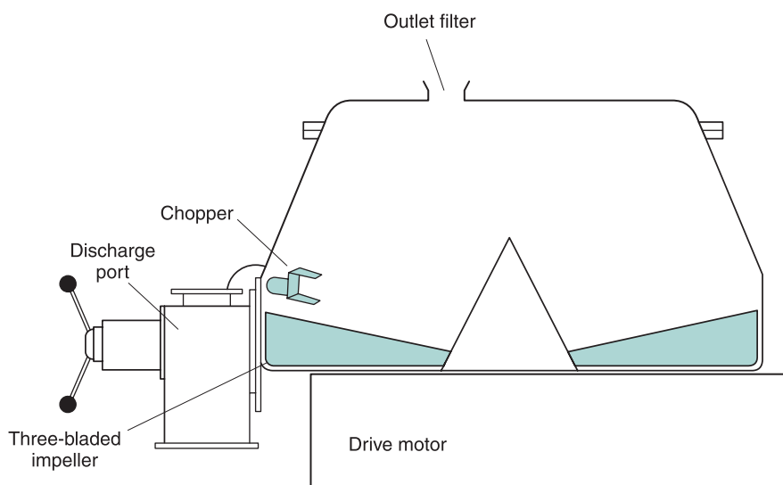
Fig. 28.4 • High-speed mixer/granulator.
