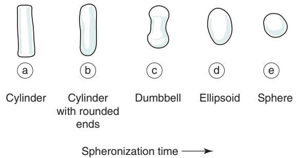
Fig. 28.10 • A spheronization mechanism, showing the transition from cylindrical particles (a) into cylindrical particles with rounded edges (b), to ellipsoids (d) and finally spheres (e).
