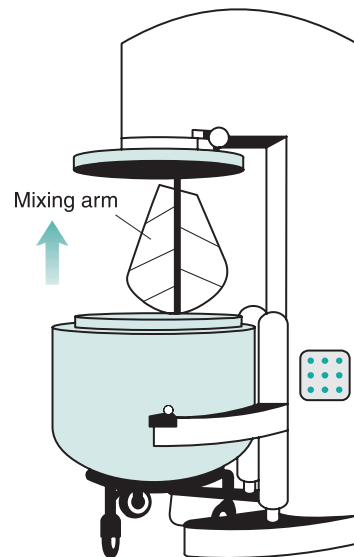
Fig.11.10 • Planetary mixer for powders and semisolids.
