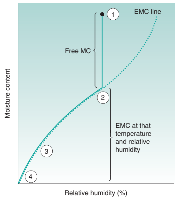
Fig. 29.2 • Loss of water from a drying solid. The wet solid before drying is at position 1. It can lose water by evaporation to position 2, its equilibrium moisture content (EMC) at that relative humidity. The only way the solid can lose more water is to reduce the relative humidity of the atmosphere, to position 3 with silica gel or to position 4 with phosphorus pentoxide. MC , moisture content.
