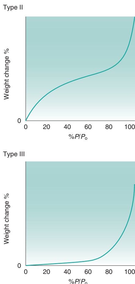
Fig. 4.5 • Type II and type III isotherms. The type II isotherm ( top ) shows weight gain as the partial pressure of the vapour ( P/P_0 ) (which would be relative humidity for water) is increased, with rapid uptake at low P/P_0 , passing through monolayer to multilayer coverage. The type III isotherm ( bottom ) shows little weight gain at low P/P_0 , with mass gain accelerating at higher P/P_0 .
