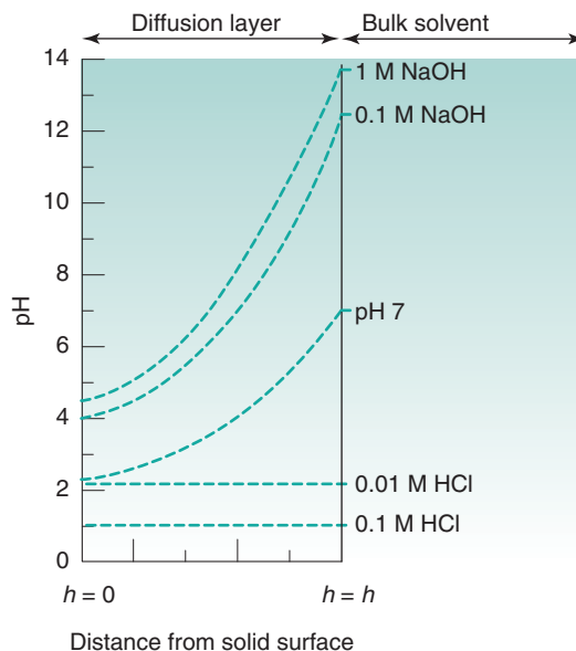
Fig. 23.11 • pH across the diffusion layer as a function of dissolution medium for salicylic acid. From Serajuddin & Jarowski, 1985.
