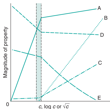
Fig. 5.12 • Solution properties of an ionic surfactant as a function of concentration, c : Osmotic pressure against c (A); solubility of a water-insoluble solubilizate against c (B); intensity of light scattered by the solution against c (C); surface tension against \log c (D); molar conductivity against \sqrt{c} (E).
