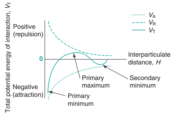
Fig. 26.3 • The energy of interaction between two similar particles, as described by the Derjaguin–Landau–Verwey–Overbeek theory.
