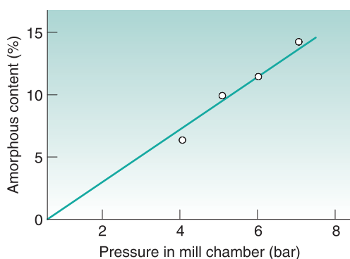
Figure 8.8 • The amorphous content induced in crystalline lactose as a consequence of milling in an air-jet mill at different air pressures. Adapted from Briggner et al., 1994 , with permission.
