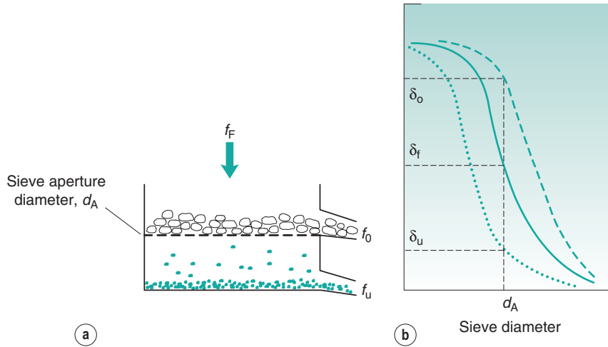
Fig. 10.16 • Size separation efficiency determination. (a) Separation operation. (b) Size distributions of feed, overflow material and underflow material to obtain values for \delta_o , \delta_f and \delta_u .
