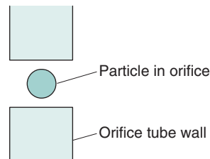
Fig. 9.14 • Particle passing through the measuring aperture of electrical sensing zone apparatus.
