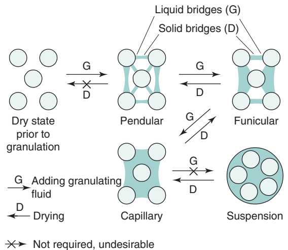
Fig. 28.2 • Water distribution between particles of a granule during formation and drying.
