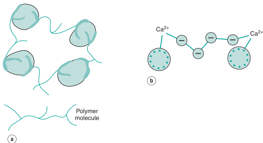
Fig. 5.6 • Floccs formed by (a) polymer bridging and (b) polyelectrolyte bridging in the presence of divalent ions of opposite charge.
