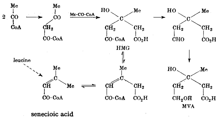
senecioic acid
