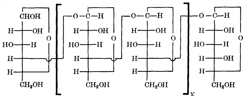
cellobiose units
