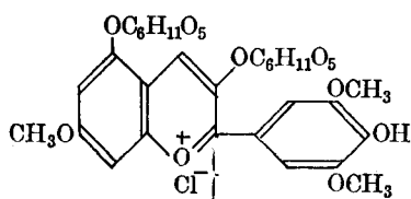
hirsutin chloride
