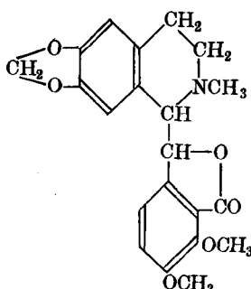
hydrastine
