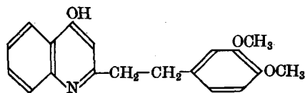
galipoline
