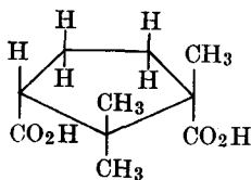
camphoric acid, m.p. 187°
