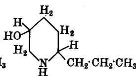
ψ-conhydrine
