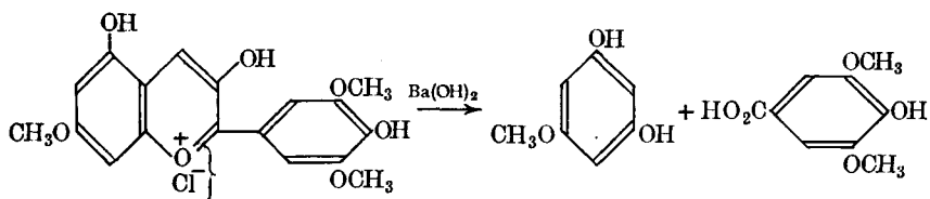
hirsutidin chloride
