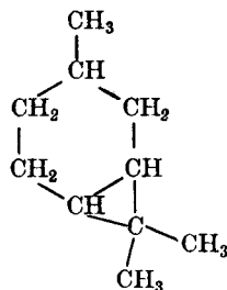
carane
