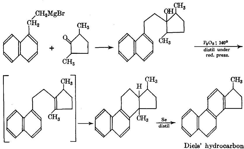
Diels' hydrocarbon
