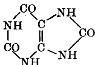
Medicus formula
