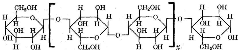
cellobiose units
