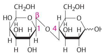
2. Lactose β-D-Galactopyranosyl-(1→4)-D-glucopyranose
