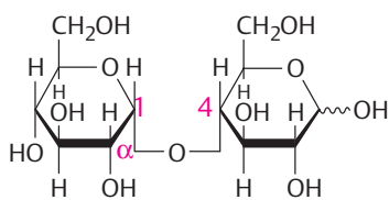
1. Maltose α-D-Glucopyranosyl-(1→4)-D-glucopyranose
