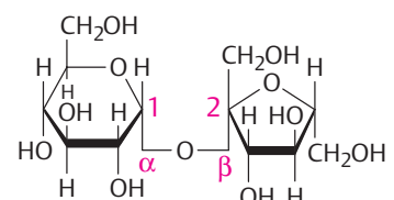
3. Sucrose α-D-Glucopyranosyl-(1↔2)-β-D-fructofuranoside
