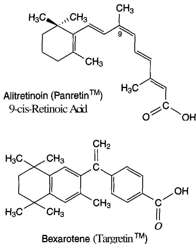
Figure 8.9. Retinoids used in the treatment of malignancies.
