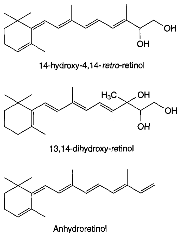
Figure 7.11. Retro-retinoids.
