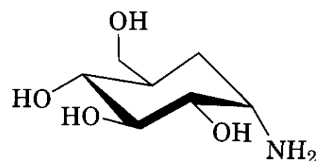
(21) validamine
