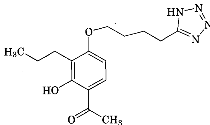
(29) tomelukast (LY 171883)
