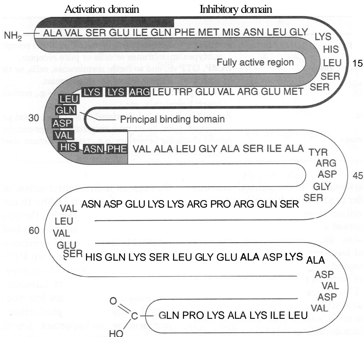
Figure 2.4. Schematic representation of the functional domains of parathyroid hormone molecule.
