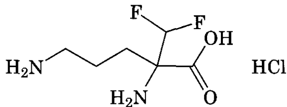
(5) Eflornithine Hydrochloride
