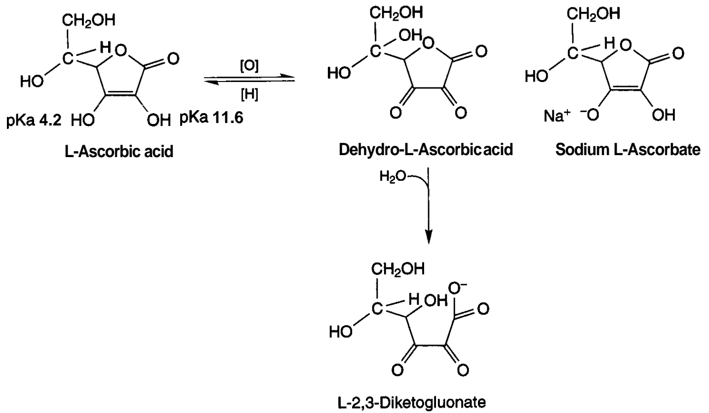
Figure 8.56. Ascorbic acid chemistry.
