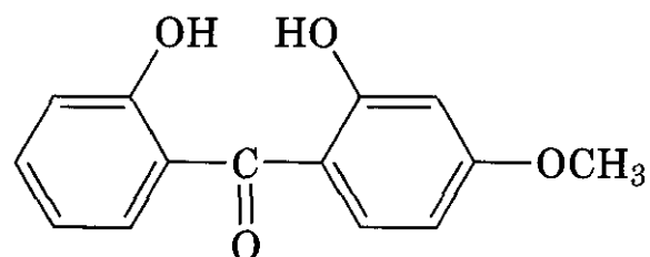
(28) Dioxybenzone (Benzophenone-8)
