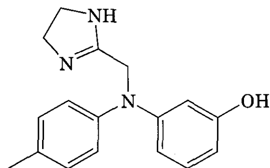
(10) Phentolamine
