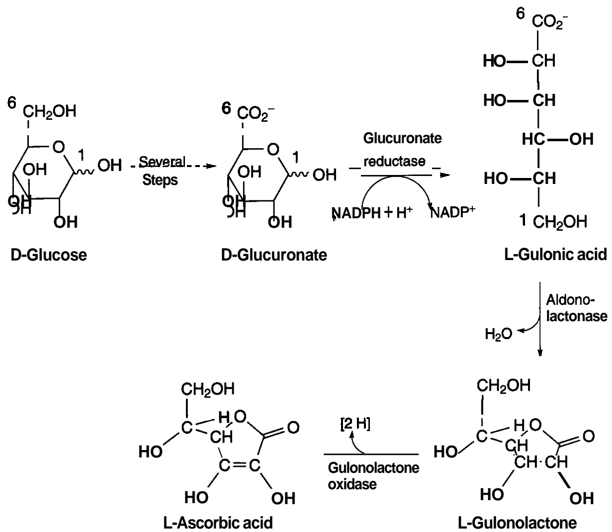
Figure 8.57. Outline of ascorbic acid biosynthesis.
