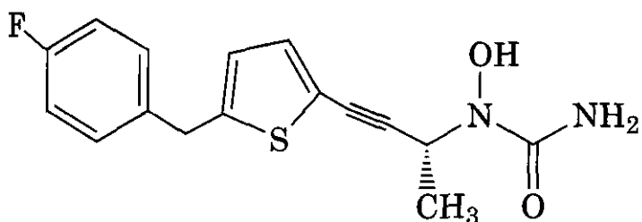
(10) ABT-761
