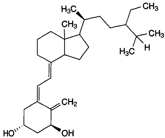
1-(OH)-24-ethyl-cholecalciferol
