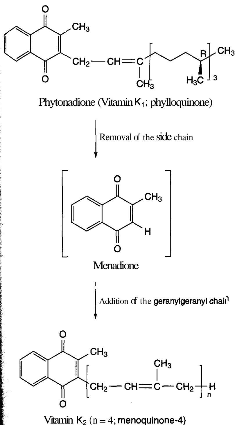
Figure 8.23. Formation of menoaquinone form of vitamin K.
