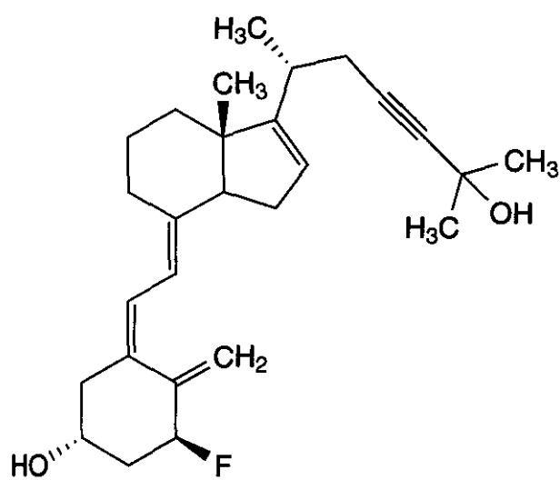
1,25-(OH) _2 -16-ene
