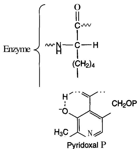
Figure 8.34. Pyridoxal phosphate bound to the enzyme.
