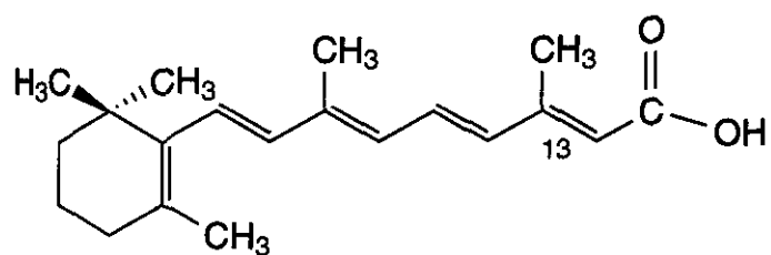
Tretinoin (Retin-A) Retinoic acid
