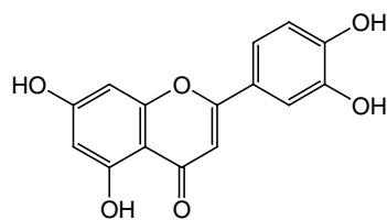
Luteolin (Flavone)
