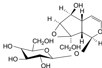
Catapol
