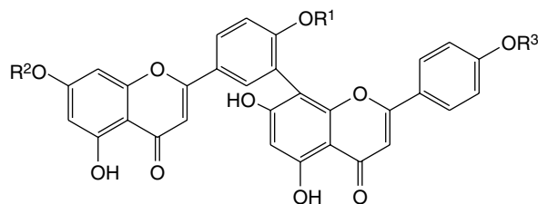
Biflavonoid structures
