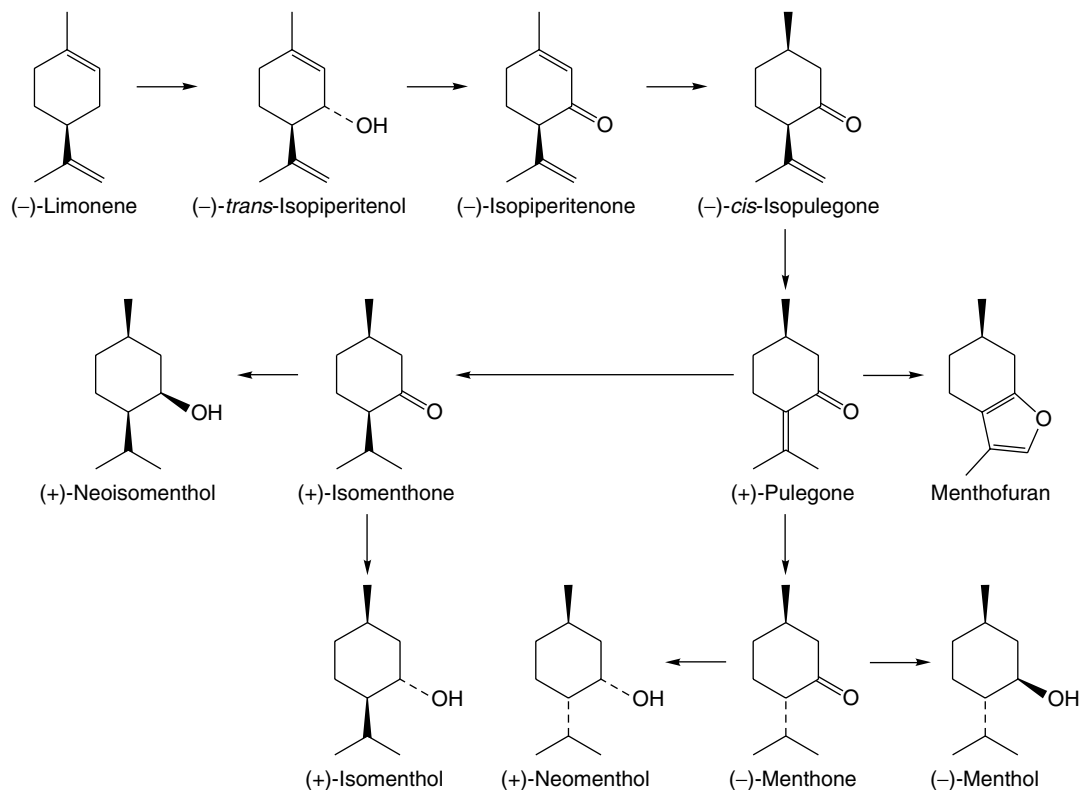
Fig. 22.3 A possible biogenetic scheme for some monoterpenoids of Mentha × piperita .
