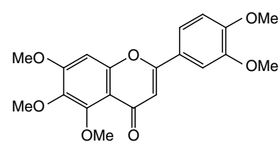
Sinensetin (Flavone)
