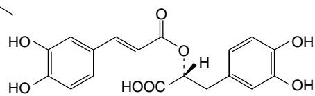
Rosmarinic acid
