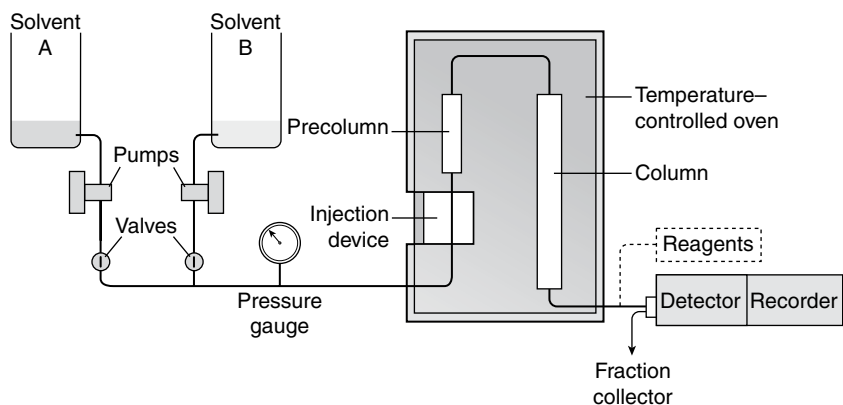
Fig. 17.1 Schematic representation of apparatus for high-performance liquid chromatography utilizing two solvents.
